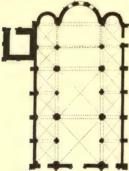
Fig. 330.—Rivolta d'Adda. Plan of church of Santa Maria e San Sigismondo XIth Century).
